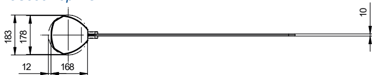
SG600 Top View
