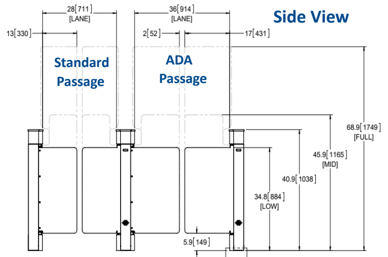
SL2000 Optical Turnstile Dimensions (28" Standard Lane with 36" ADA Lane)
