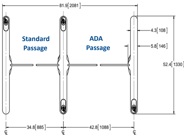
SL2000 Optical Turnstile Dimensions (28" Standard Lane with 36" ADA Lane)
