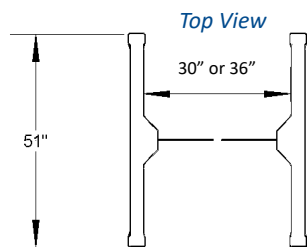
SG-2 High Glass Optical Turnstile Standard Dimensions (single lane)
